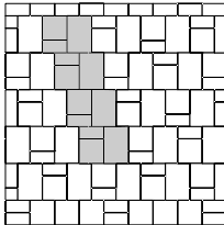
Pattern 5 Two full layers
