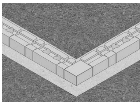
90° Outside Corner Base Course
