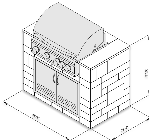
32" Sizzler Pro Grill Cabinet
