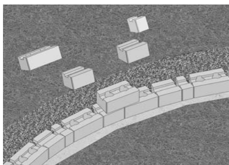
Building a Concave Curve
