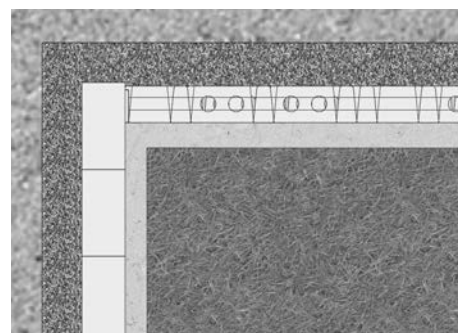
Capping a 90° inside corner
