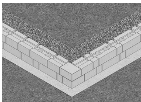
90° Outside Corner Second Course
