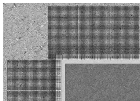
Reinforcing a 90° Inside Corner
