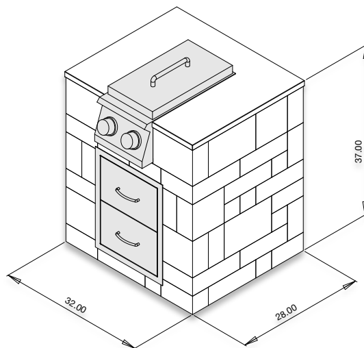
Side Burner Cabinet
