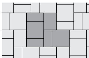
Arcana D - 46% 24" x 24", 18% 18" x 24", 36% 12" x 24"
