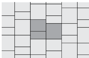
Arcana B - 44% 24" x 24", 33% 18" x 24", 23% 12" x 24"
