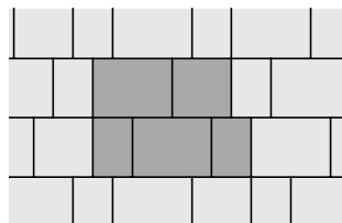
Richcliff D - 53% 12" x 9", 20% 9" x 9", 27% 6" x 9"
